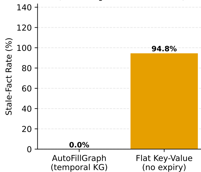
Stale-Fact Rate (conflicting values across docs)
