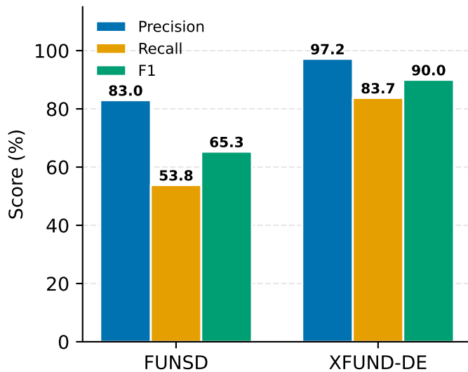
KB Triple Metrics (Precision / Recall / F1)
