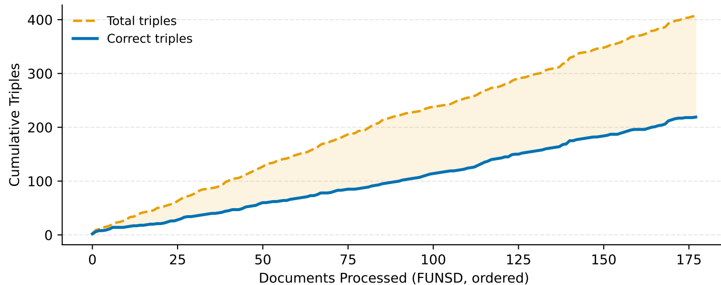
KB Growth Curve — Cumulative Triples Accumulated
